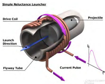
Fig. 2. Coil Gun Principle
