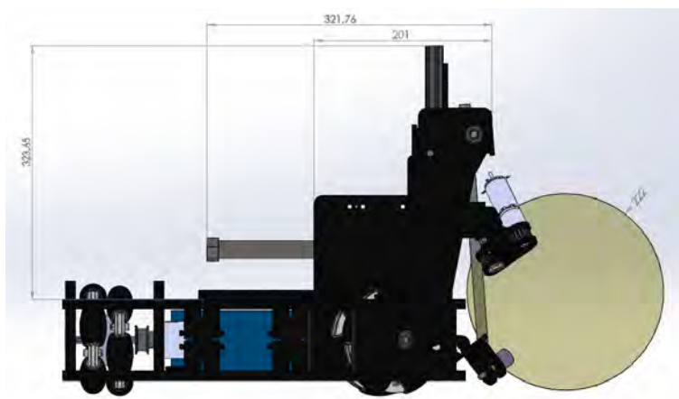
Fig. 1. Kicking system in a RoboCup robot
