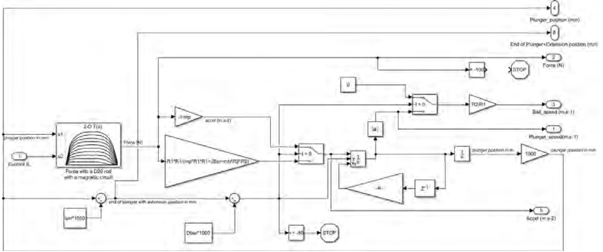
Fig. 13. Mechanical part of the coil gun model
