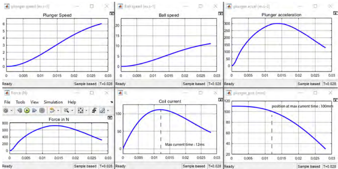
Fig. 15. Simulation using Tech United [6] one phase configuration
