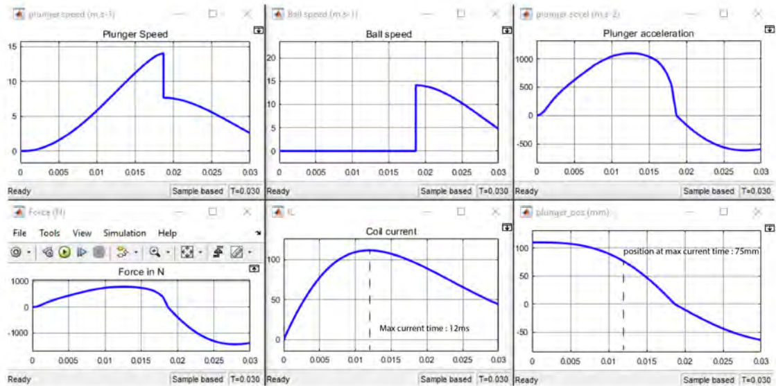
Fig. 16. Simulation using the optimal three phases configuration
